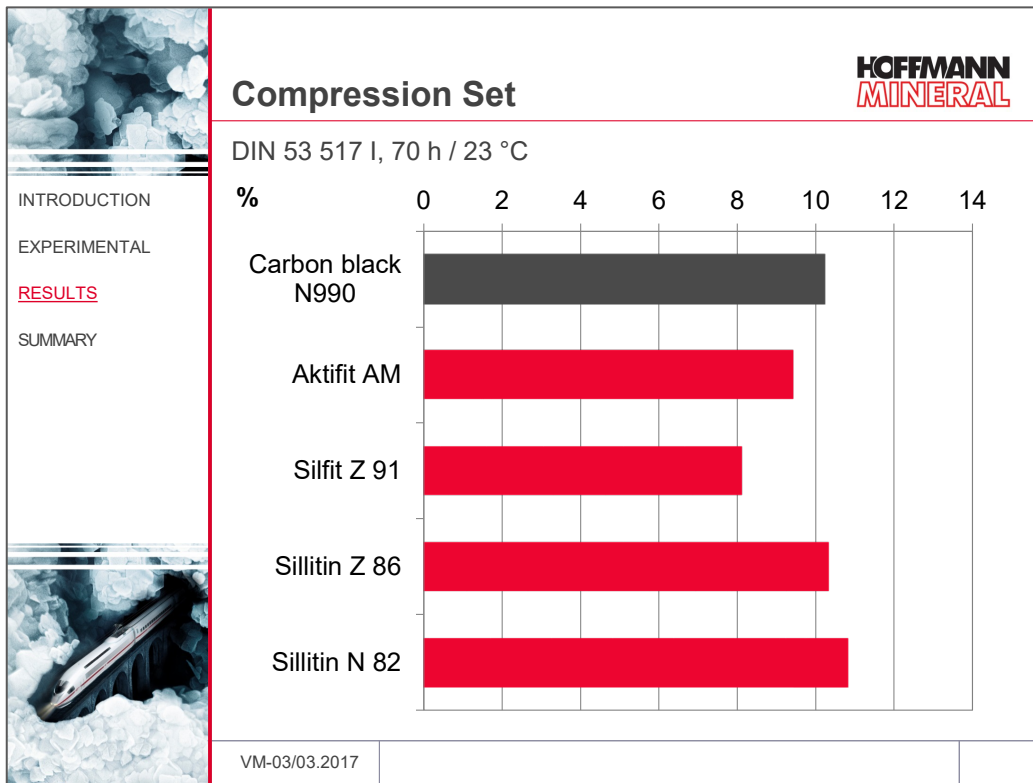
Fig. 17 By comparison, the compression set at 23 °C with Aktifit AM and Silfit Z 91 shows up even better than with carbon black N990. With Sillitin grades, the results hardly differ from the straight carbon black compound (Fig. 17).
