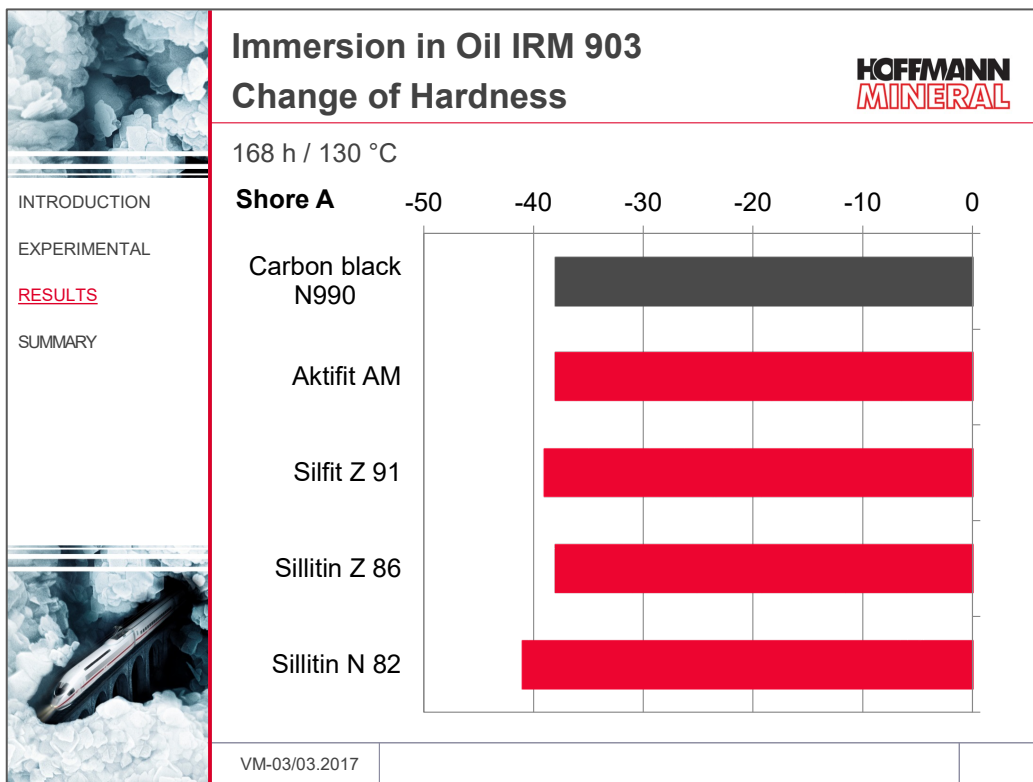
Fig. 18 Further tests evaluated the resistance against the aggressive standard oil IRM 903, i.e. under demanding conditions for an EPDM compound. Hardness decreased for all compounds to an equal extent, only Sillitin N 82 shows a somewhat bigger change (Fig. 18).
